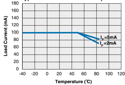
CPC1017N Typical Load Current vs. Temperature
