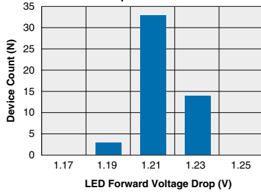
CPC1017N Typical LED Forward Voltage Drop (Ambient Temperature = 25°C) I_F = 5\text{mADC}
