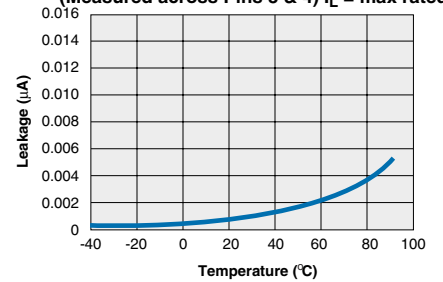
CPC1017N Typical Leakage vs. Temperature (Measured across Pins 3 & 4) I_L = \text{max rated}
