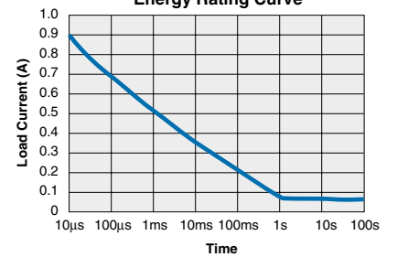
CPC1017N Energy Rating Curve
