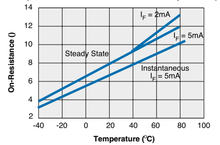
CPC1017N Typical On-Resistance vs. Temperature (Load Current = max rated @ temperature)
