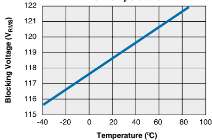
CPC1017N Typical Blocking Voltage vs. Temperature
