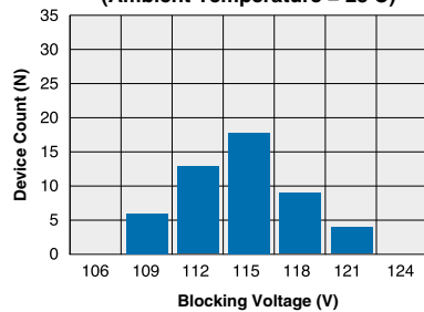
CPC1017N Typical Blocking Voltage Distribution (Ambient Temperature = 25°C)
